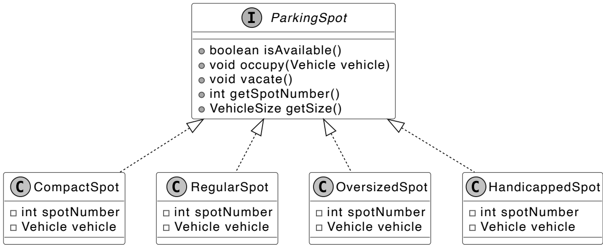
ParkingSpot with HandicappedSpot class
