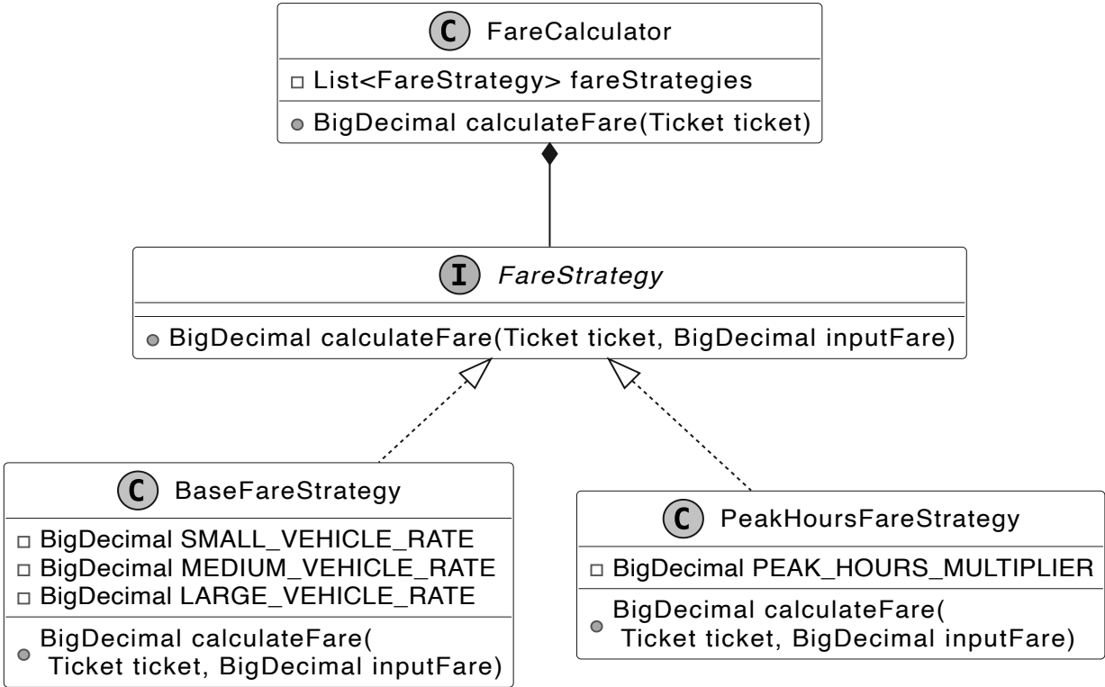
FareStrategy interface and FareCalculator class
